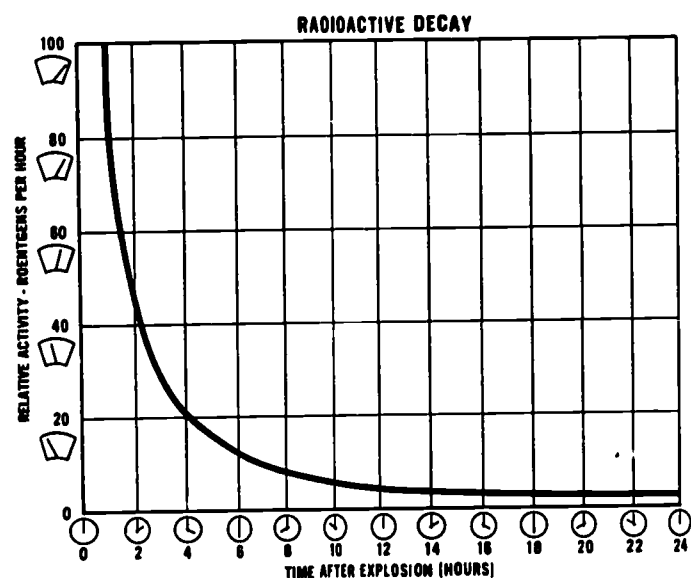
FIGURE 9.—Radioactive Decay
